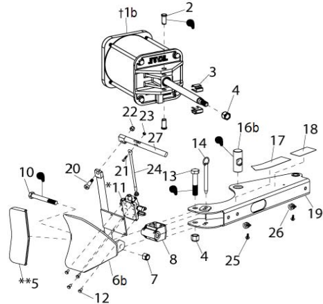
B.L. Arm Assembly - Hand Operated
