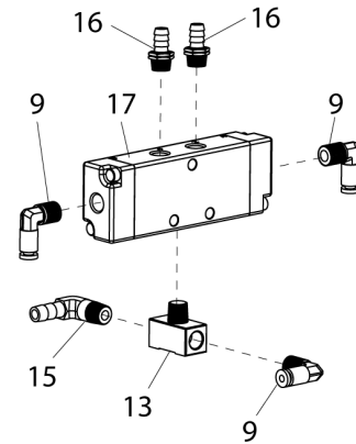
Pilot Valve Assembly
