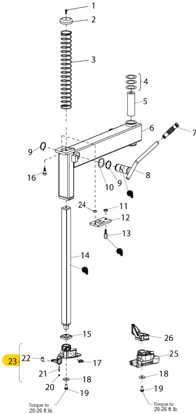
Steel DuckHead® Mount/Demount Tool
