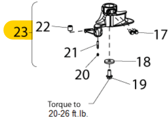
Steel DuckHead® Mount/Demount Tool
